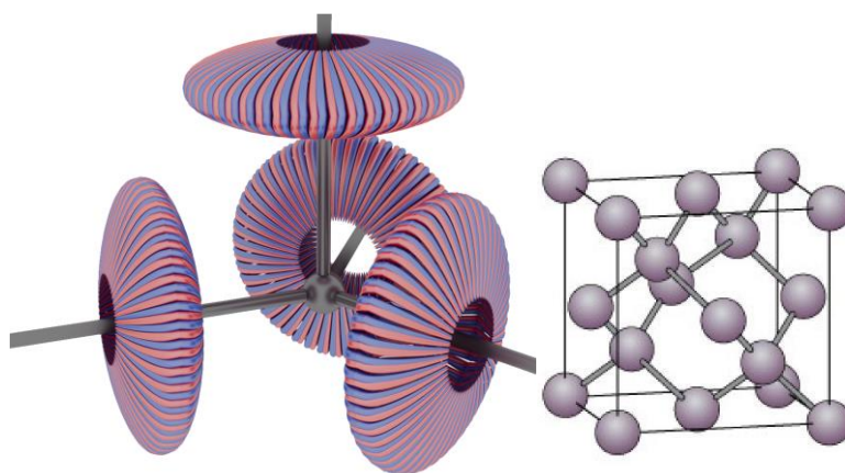
Figure 28. Tetravalent covalent electronic structure of carbon in the crystal lattice of diamond
