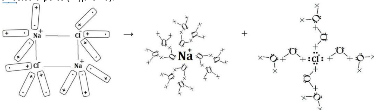
Figure 16. Dissociation of sodium chloride
