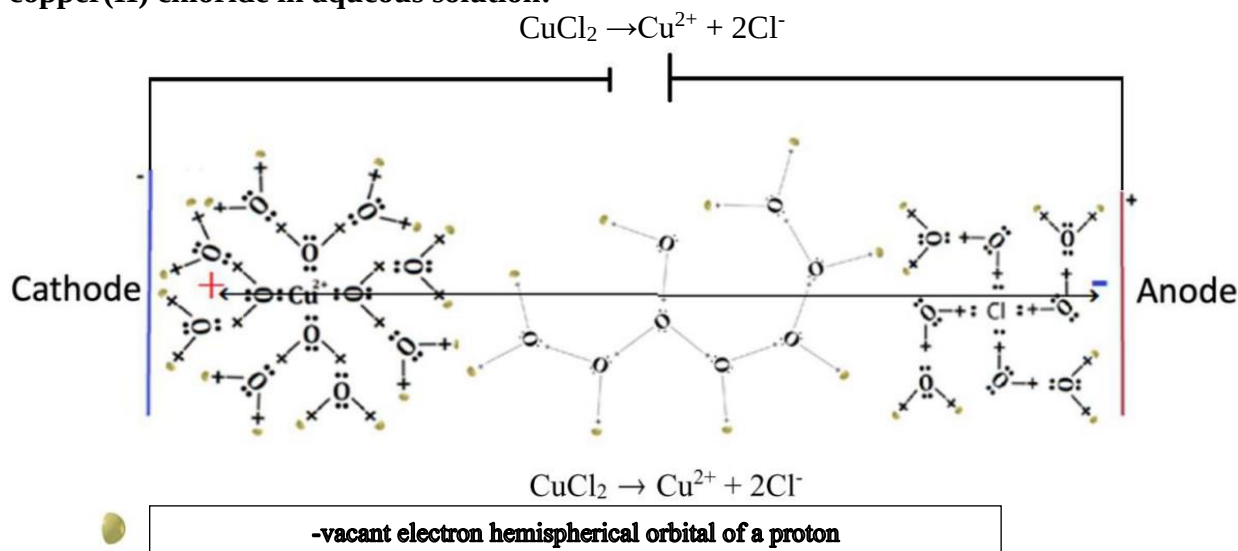
Figure 18. Scheme of the electrolysis of a solution of copper(II) chloride
