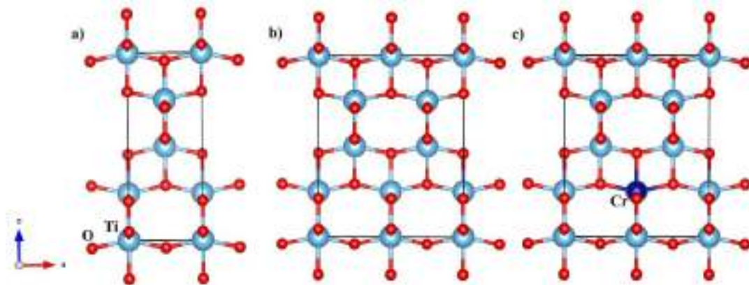
Fig1. Anataza TiO 2 ning elementar yacheykasi (a) Cr doped qilinmasdan oldingi (b) Cr doped qilingandan keyingi superyacheykalari (c).
