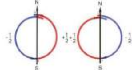
Fig. 3. Toroidal cross-section of the spin of the electron EMWP in a magnetic field in the free state
