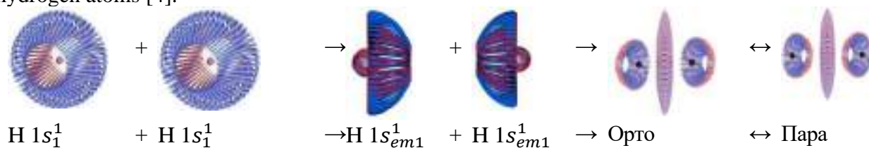
Fig. 8. Formation of ortho- and para-positronic molecular hydrogen
