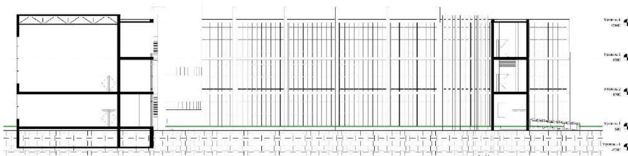
2-rasm. Maktab binosining qirqimi
