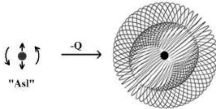
Figure 3. Neutron formation
