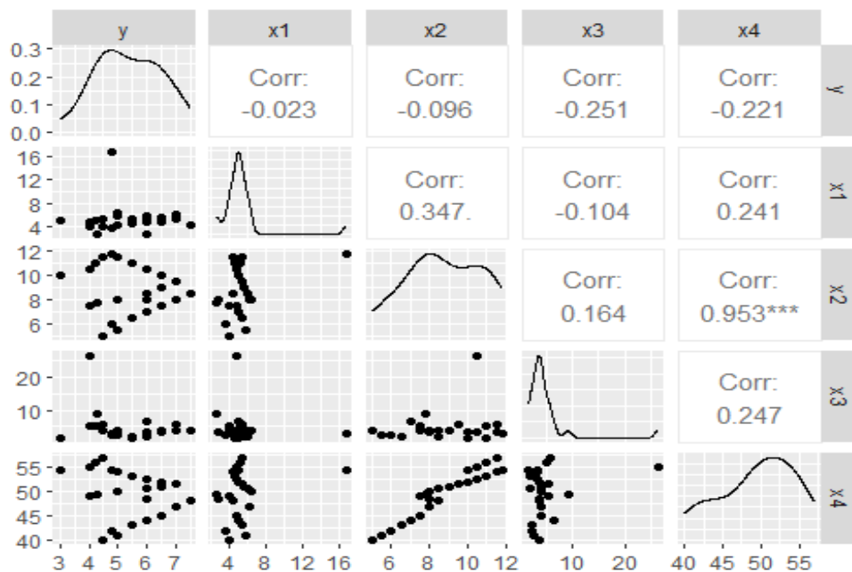
Graph 1. Graphical representation of the correlation matrix
