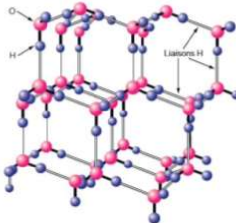
Figure 9. Crystal structure of water
