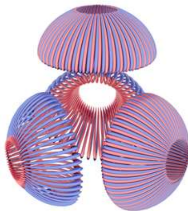
Figure 2. Outer electron shell of the oxygen atom ( 2s^2_{ec1} 2s^2_{ec2} 2s^1_{ec3} 2s^1_{ec4} )
