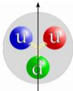
Fig. 4. Spatial Arrangement of the Two u-Quarks and One d-Quark within the Proton, Together with the Axis of Its Magnetic Dipole Moment
