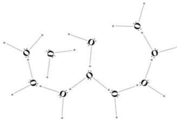
Figure 8. Polymolecular network cluster structure containing individual water molecules
