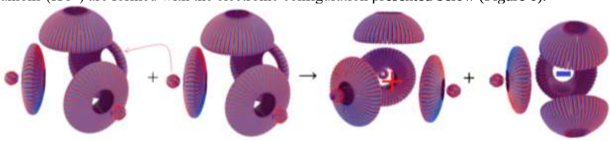
Figure 6. Electron-configuration model of the formation of H_3O^+ and HO^- ions according to the transformation theory
