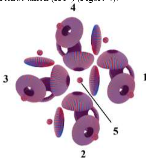
Figure 4. Initial spatial configuration of proton separation from the water molecule according to the EMWP model.
