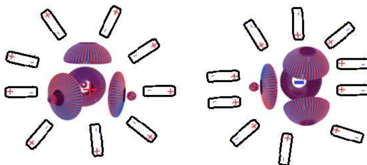
Figure 7. Hydrated state of hydronium and hydroxide ions
