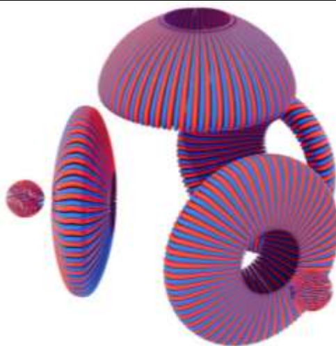
Figure 3. Spatial configuration of the water molecule according to the EMWP model
