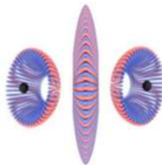
Para-Proton Configuration
