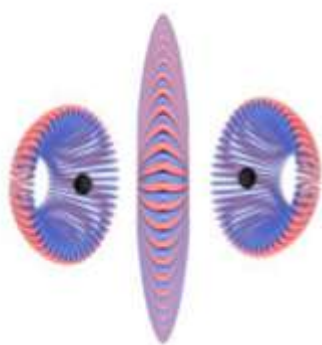
Ortho-Proton Configuration
