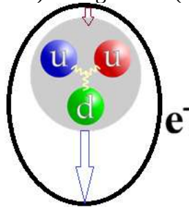
Fig. 2. Schematic Illustration of the Electrostatic Influence of the Proton's Quark Structure on the Configuration of the Electron Orbital
