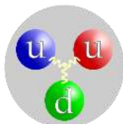
Fig. 1. Structure of the Proton
