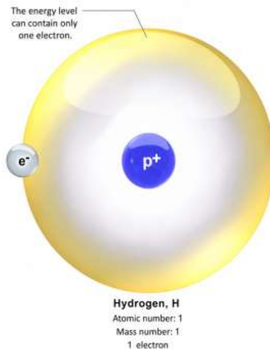
Fig. 3. Composition and Structure of the Hydrogen Atom
