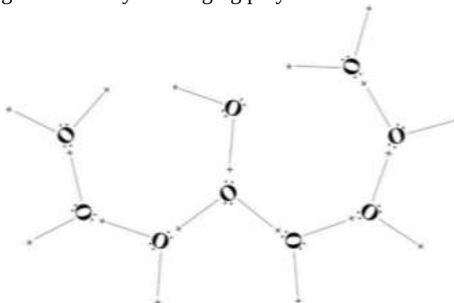
Figure 5. Polymolecular cluster network structure of water
