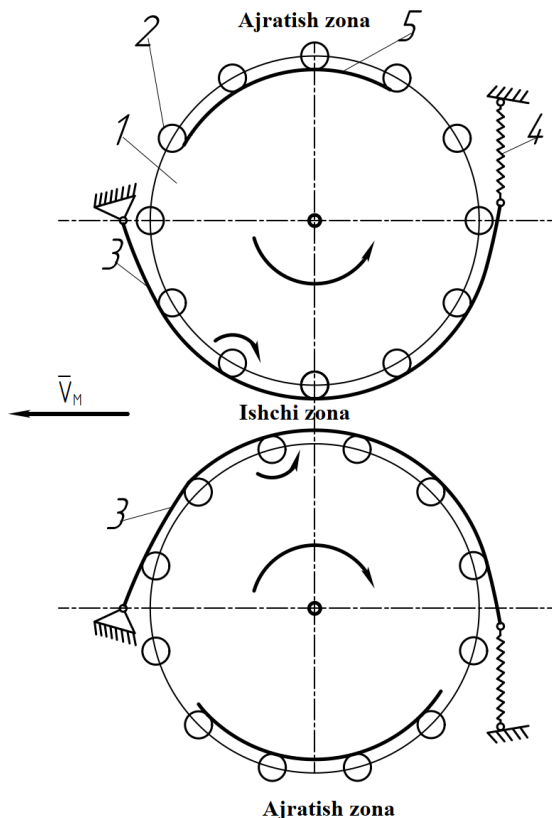
1-rasm. Shpindelni aylantiradigan friktsion yuritma sxemasi: 1- shpindelli baraban; 2-shpindel; 3- terish zonasidagi tashqi oddiy ponasimon tasmalar; 4-tortib turuvchi prujina; 5-ajratish zonasidagi ichki tasmalar.
