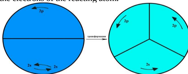
Fig. 3. Transformation of electrons in a boron atom
