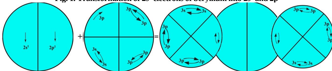
Fig. 2. Formation of a beryllium chloride molecule
