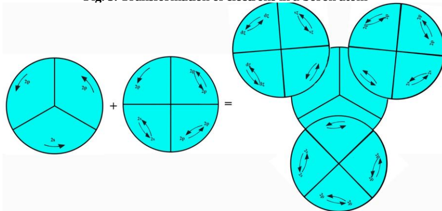
Fig. 4. Formation of a boron fluoride molecule
