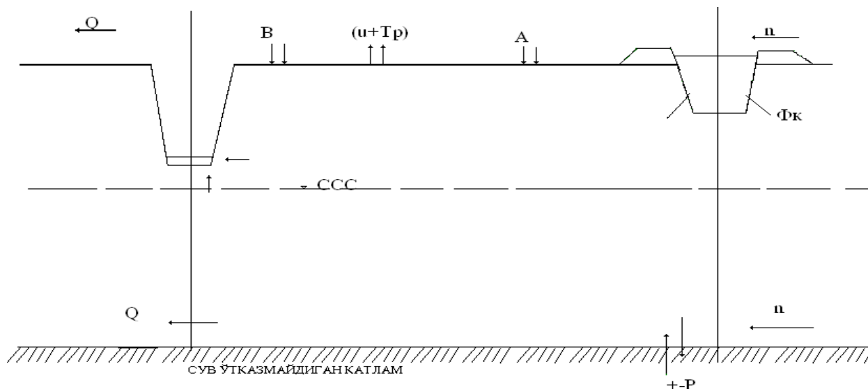
Figure 1. Equilibrium scheme of the field.
