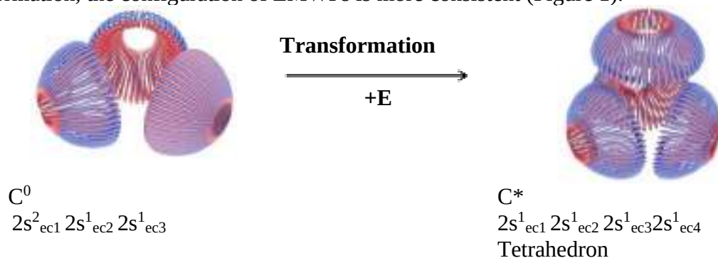
Figure 1. Transformation of the electromagnetic orbitals of a carbon atom upon excitation
