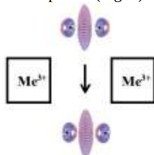
Fig. 9. Transition of ortho-hydrogen to para-hydrogen under the influence of metal ions
