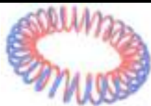
Fig. 1. EMWP electron in the free state
