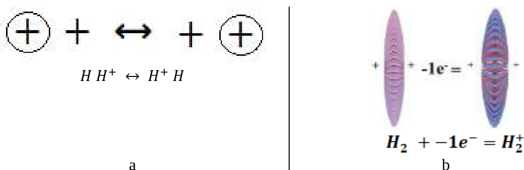
Figure 7. Formation of molecular hydrogen ion: a) classical method, b) transformation theory method
