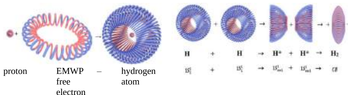
a) Formation of a hydrogen atom
