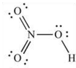
Figure 4. Nitric acid (HNO 3 ): Nitrogen valence is 5, Oxidation state is +5.
