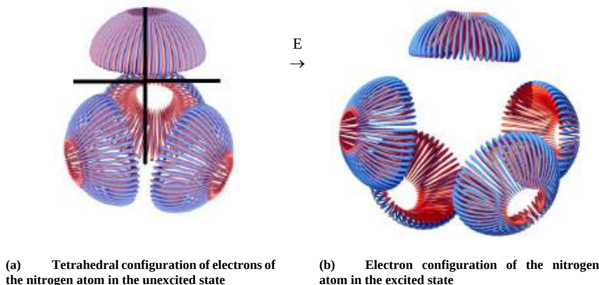
Figure 1. Transition of a nitrogen atom to an excited state with the opening of a vacant sector for electrons and the appearance of unpaired electrons.
