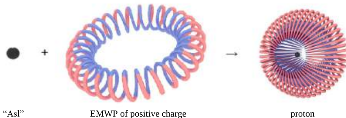
Figure 5. Formation of a proton
