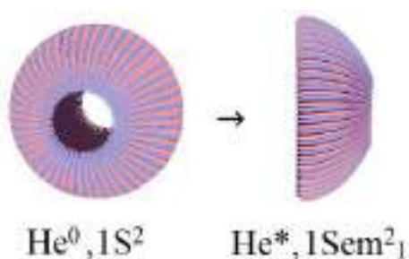
Figure 14. Transformation of paired electrons of parahelium
