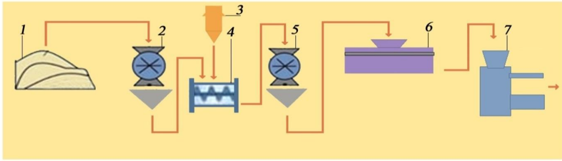
Fig. 1. Technological scheme of activation of the natural clay mineral kaolin Sultan-Uvays 1. Natural clay mineral kaolin Sultan-Uvays. 2. Kaolin mineral grinder. 3. Drinking water storage tank. 4. Furnace for heating the mineral kaolin. 5. Kaolin adsorbent grinder. 6. Separator. 7. Apparatus for packing the finished adsorbent.
